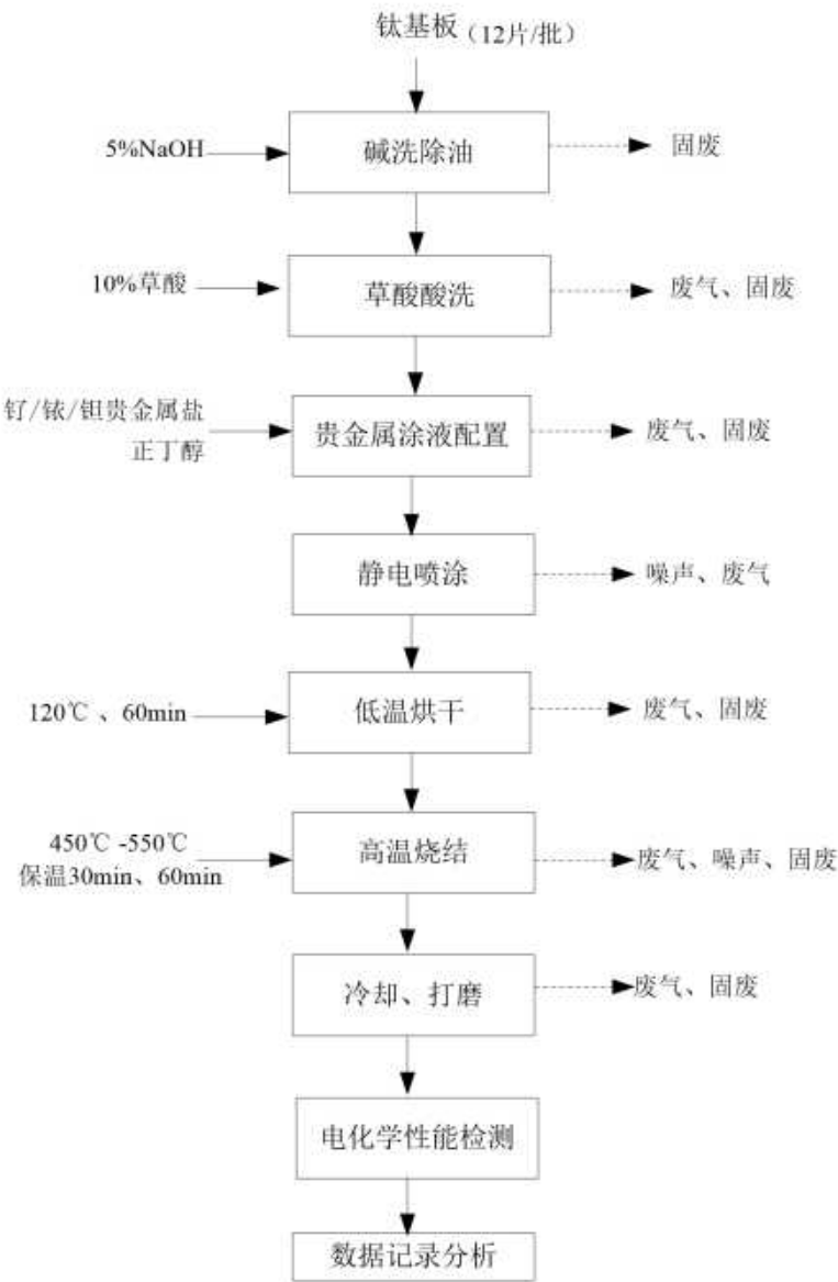
图2-4 钛阳极制备及性能评价流程图
